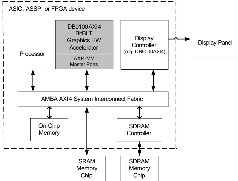
Figure 1: DB9100AXI4 BitBLT Graphics HW Accelerator – System Diagram
